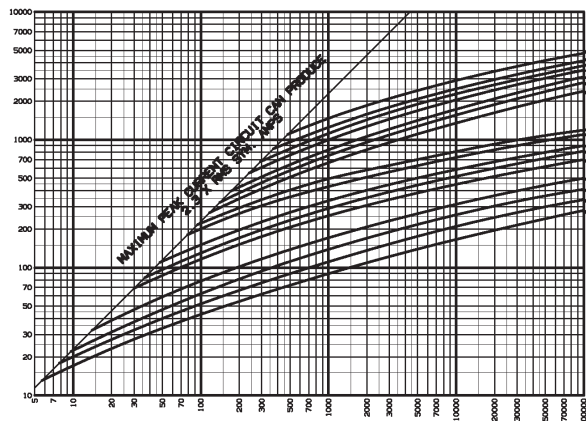
Peak Let-Through Current Data
