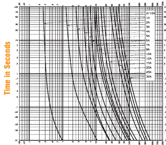
Melting Time – Current Data
